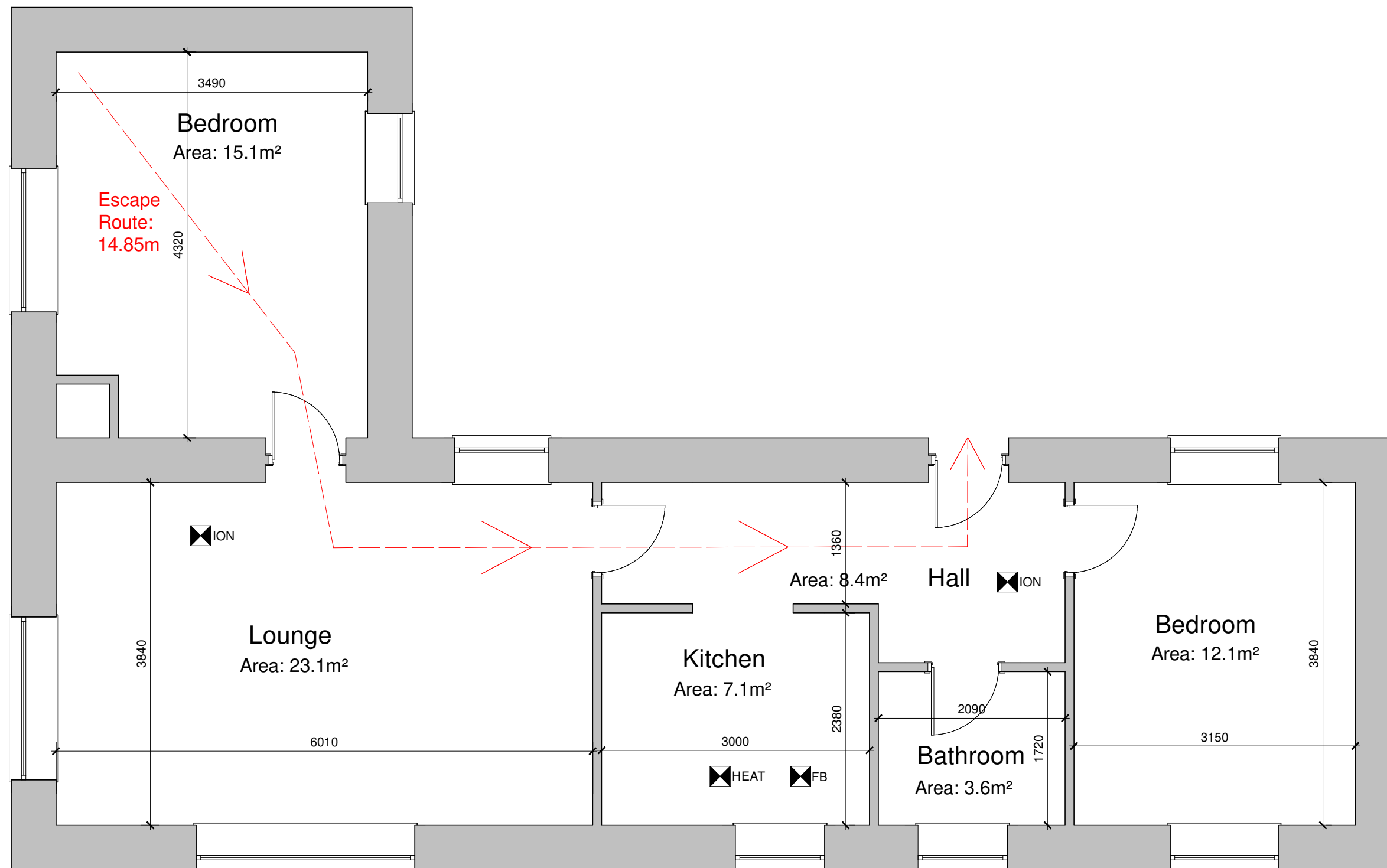
Ground Floor Plan at Scale 1:50 Total Internal Floor Area = 72.6m²
